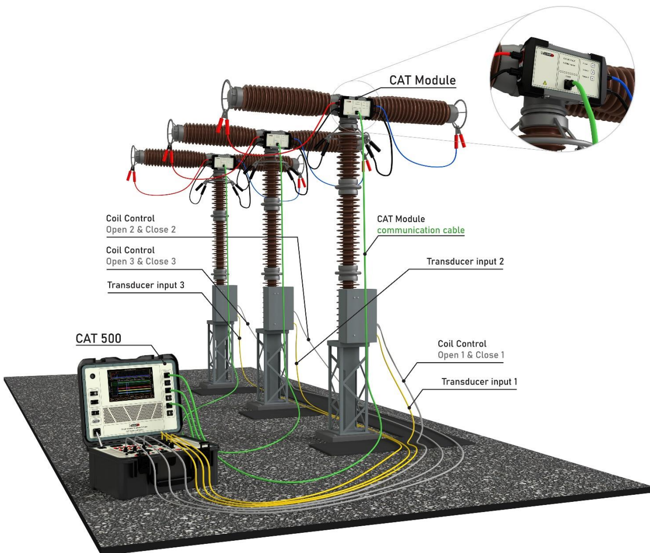
Simultaneous timing, contact resistance and dynamic resistance measurement of up to 6 interrupting chambers
