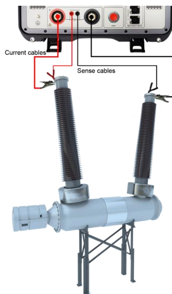
Micro Ohmmeter cable connection on a dead tank circuit breaker
