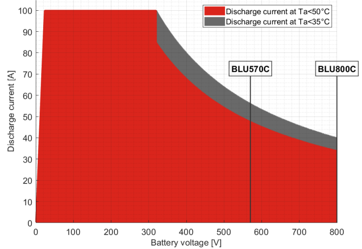
BLU570C and BLU800C - Maximum discharge current VS Battery voltage
