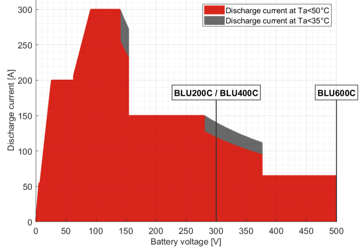
BLU200C, BLU400C and BLU600C - Maximum discharge current VS Battery voltage
