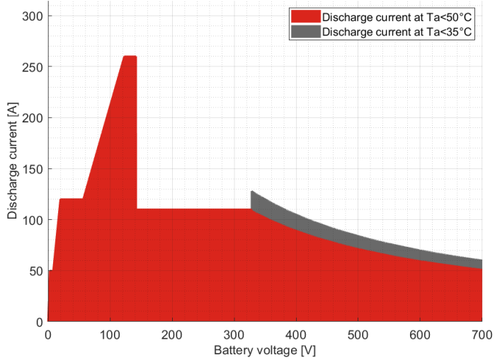
BLU700C - Maximum discharge current VS Battery voltage
