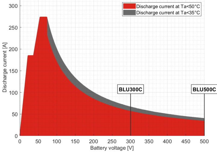
BLU300C and BLU500C - Maximum discharge current VS Battery voltage
